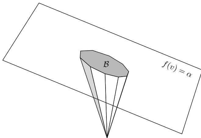
Figure 3.4: A visualization of Theorem 3.12.
